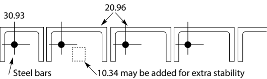
200 mm clean out course for 20.91
