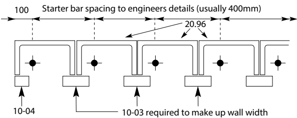
30.48 clean out course and starter bar spacing
