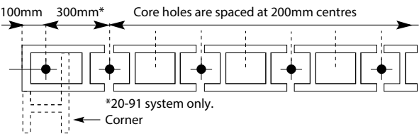
Core spaces at ends and corners for 20.91 systems
